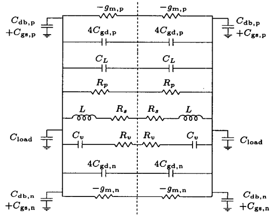
Figure 3: Complementary LC oscillator.
