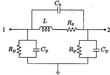
Figure 2: Simplified inductor model.
