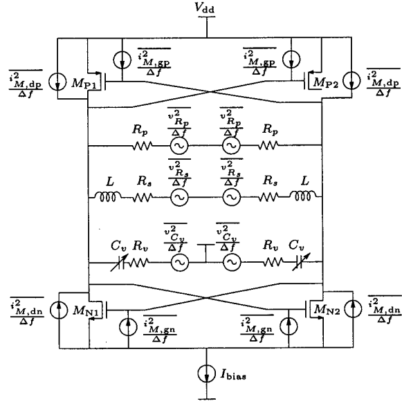
Figure 4: Noise sources in the LC oscillator.
