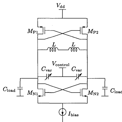
Figure 1: Complementary LC oscillator.
